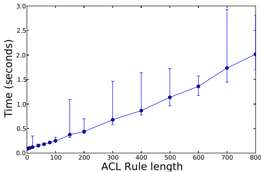
Figure 7: Performance on checking individual firewalls.
