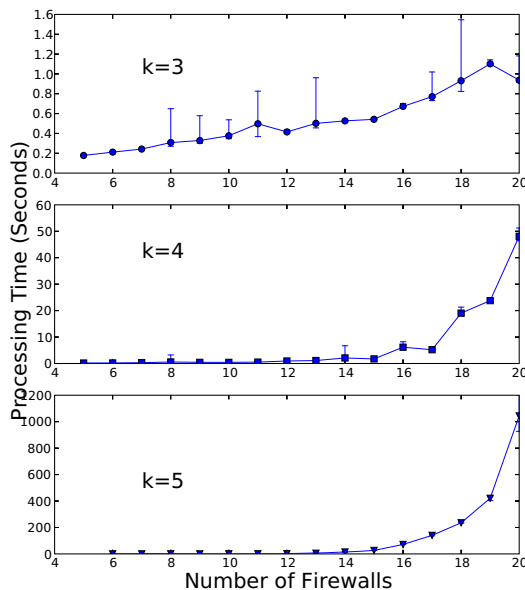
Figure 8: Performance on checking distributed firewalls.
