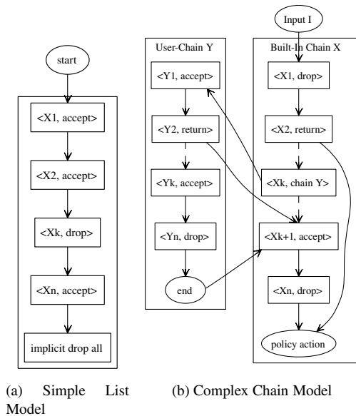
Figure 1: Model of individual firewalls.
