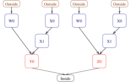
Figure 4: ACL tree.
