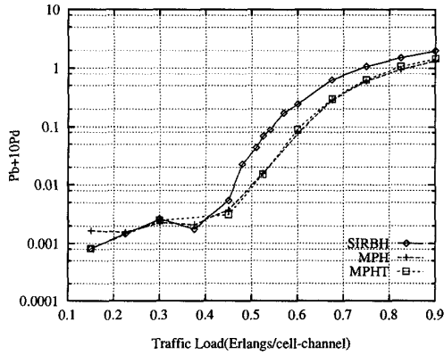
Figure 3: Combined Performance Measures ( \gamma_{drop}=16\text{dB} , \gamma_t=19\text{dB} , \gamma_{new}=22\text{dB} , \text{OUTAGE}=0 )
