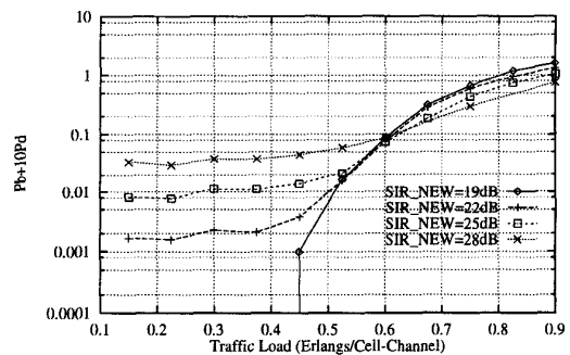
Figure 7: Combined Performance Measures for MPH as a function of \gamma_{new} (SIR_NEW) ( \gamma_{drop}=16\text{dB} , \gamma_t=19\text{dB} , \text{OUTAGE}=0 )
