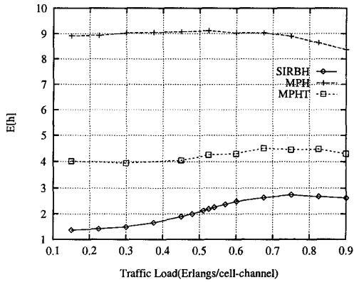
Figure 4: Mean Number of Handoffs per Call vs. Load ( \gamma_{drop}=16\text{dB} , \gamma_t=19\text{dB} , \gamma_{new}=22\text{dB} , \text{OUTAGE}=0 )
