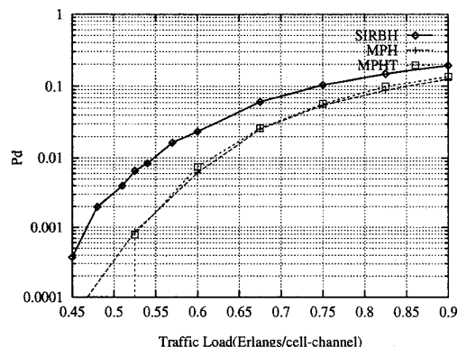
Figure 2: Dropping vs. Load ( \gamma_{\text{drop}}=16\text{dB} , \gamma_t=19\text{dB} , \gamma_{\text{new}}=22\text{dB} , OUTAGE=0)
