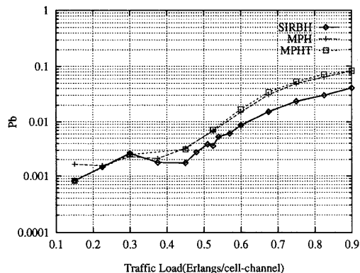
Figure 1: Blocking vs. Load ( \gamma_{\text{drop}}=16\text{dB} , \gamma_t=19\text{dB} , \gamma_{\text{new}}=22\text{dB} , OUTAGE=0)
