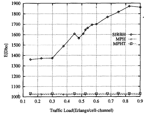
Figure 5: Mean Handoff Distance from Old Base Station as a Function of Traffic Load ( \gamma_{drop}=16\text{dB} , \gamma_t=19\text{dB} , \gamma_{new}=22\text{dB} , \text{OUTAGE}=0 )
