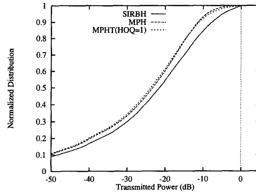
Figure 6: Normalized CDF of Power Transmitted by all users throughout the simulation ( \gamma_{drop}=16\text{dB} , \gamma_t=19\text{dB} , \gamma_{new}=22\text{dB} , \text{OUTAGE}=0 )
